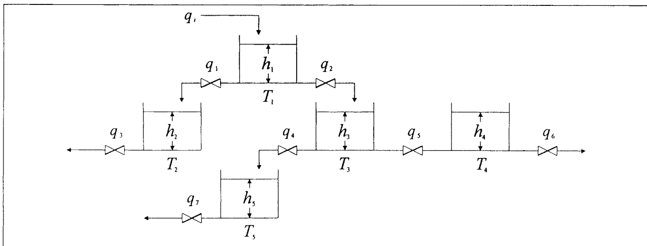
Figure 15. Simplified process flow diagram of a five-tank system.
