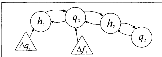
Figure 6. Precedence diagram of the two-tank system in Figure 1.
